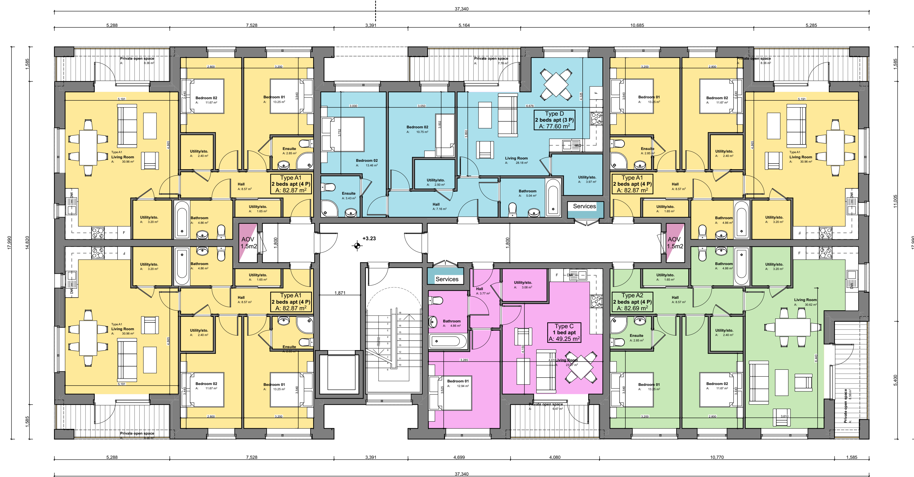
1:100 GF Ground Floor
